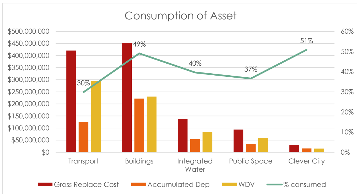
Figure 25: Asset Consumption
